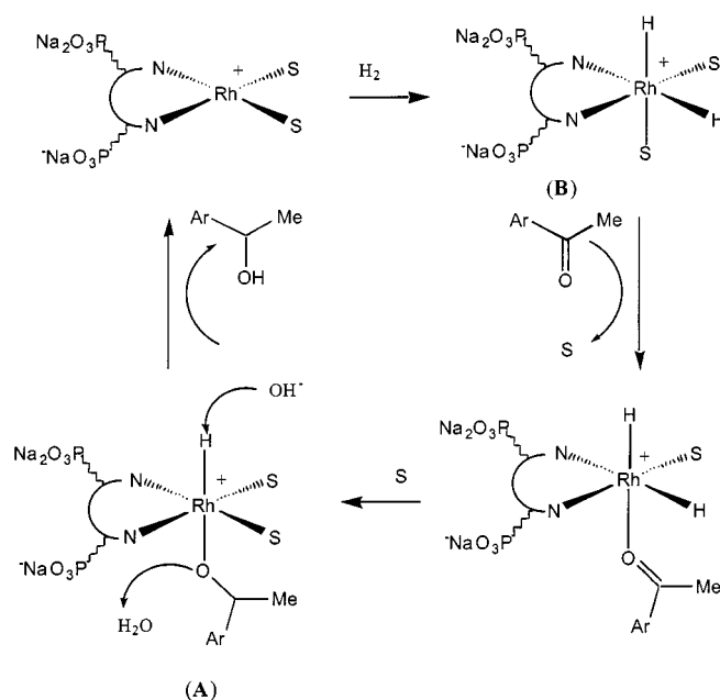
Scheme 3. Proposed effect of NaOH in the catalytic site of Rh-catalyzed hydrogenation of ketones in water under hydrogen pressure; S = H 2 O
