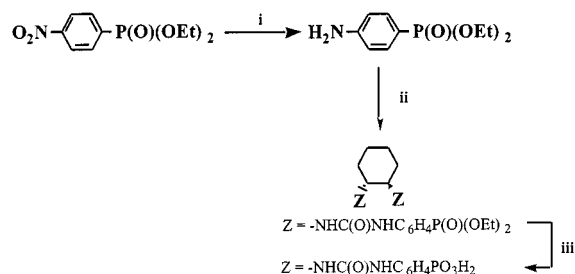
Scheme 2. Conditions: i) 5% Pd/C, HCO 2 H, NEt 3 (82%); ii) (CCl 3 O) 2 CO, NEt 3 , CH 2 Cl 2 , then (1 R ,2 R )-diaminocyclohexane (75%); iii) Me 3 SiBr, CH 2 Cl 2 , room temp., then MeOH, room temp., (quant.)
